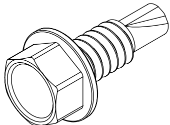
1/4"-14 X 1" HARDENED STEEL SELF-DRILLING SCREW
