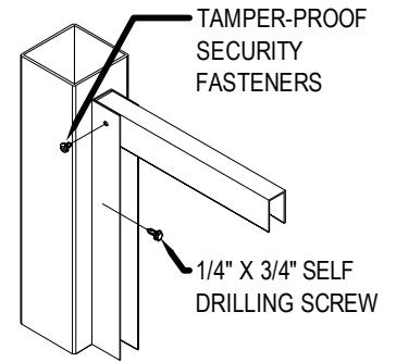
CHANNEL ATTACHMENT
