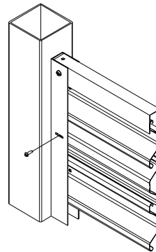
ALTERNATE PICKETS FASTEN EACH END
