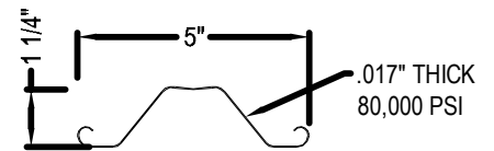
PICKET
